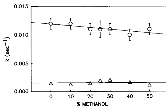
Fig.1. Effect of methanol on the kinetics of slow refolding ribonuclease A. The kinetics were measured by the change in absorbance at 286 nm. Conditions: pH* 3.0, 0.5^{\circ}\text{C} . Data for (○) faster slow refolding, (Δ) slower phase.
